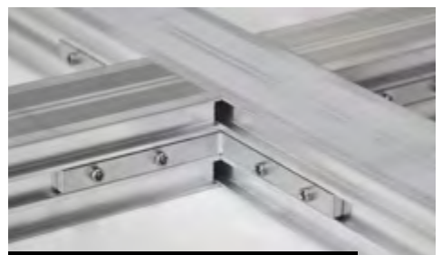
RELO E Corner brackets for frame construction
