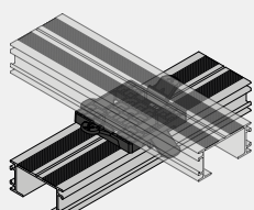
with RELO C56 62 mm build-up height*
