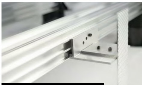
RELO BS Deck fascia bracket set for RELO substructure
